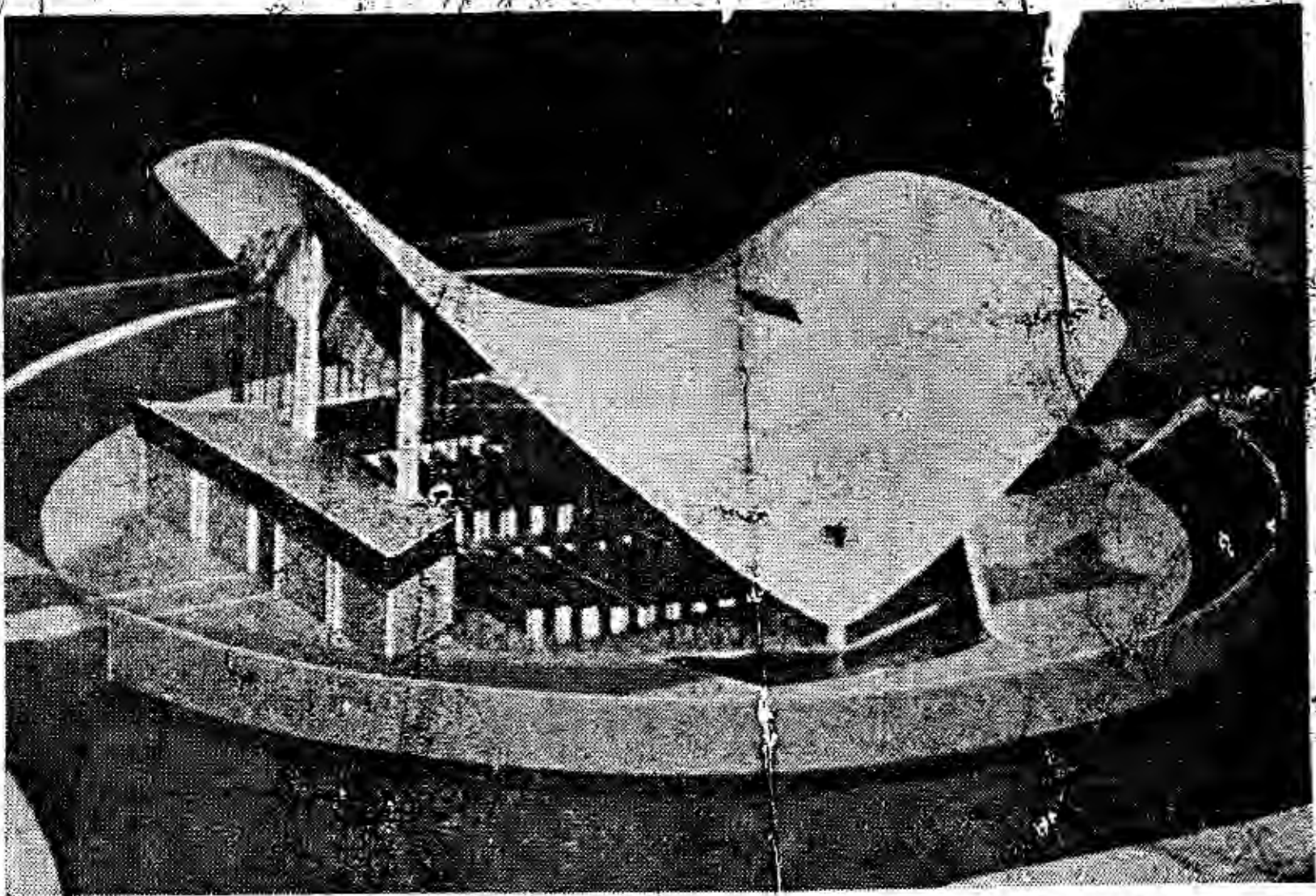
This is a preliminary model of the proposed St. John's Church, Ermine Estate, Lincoln, designed by Mr. Sam Scorer, the Lincoln architect. The all-concrete roof will have no internal pillars. The external struts shown in the picture here will be filled in with bricks and glass. (See Page 5).
